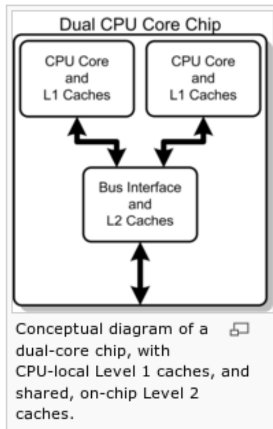
Abbildung 1.27: Dual-core CPU
