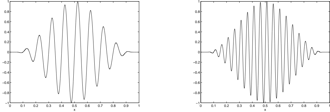
Figure 1: Modulated initial function (3.36) for p = 10 and p = 20 .
