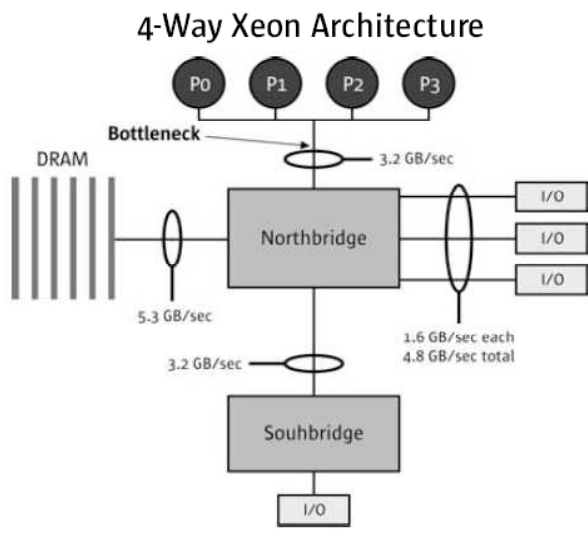
Abbildung 1.24: Hypertransport-Link vs. FSB
